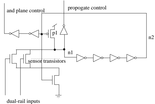
Fig. 5. PLA controller
